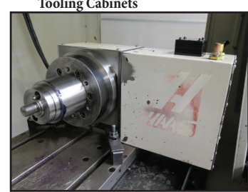
Haas 4th Axis 8" Rotary Table
